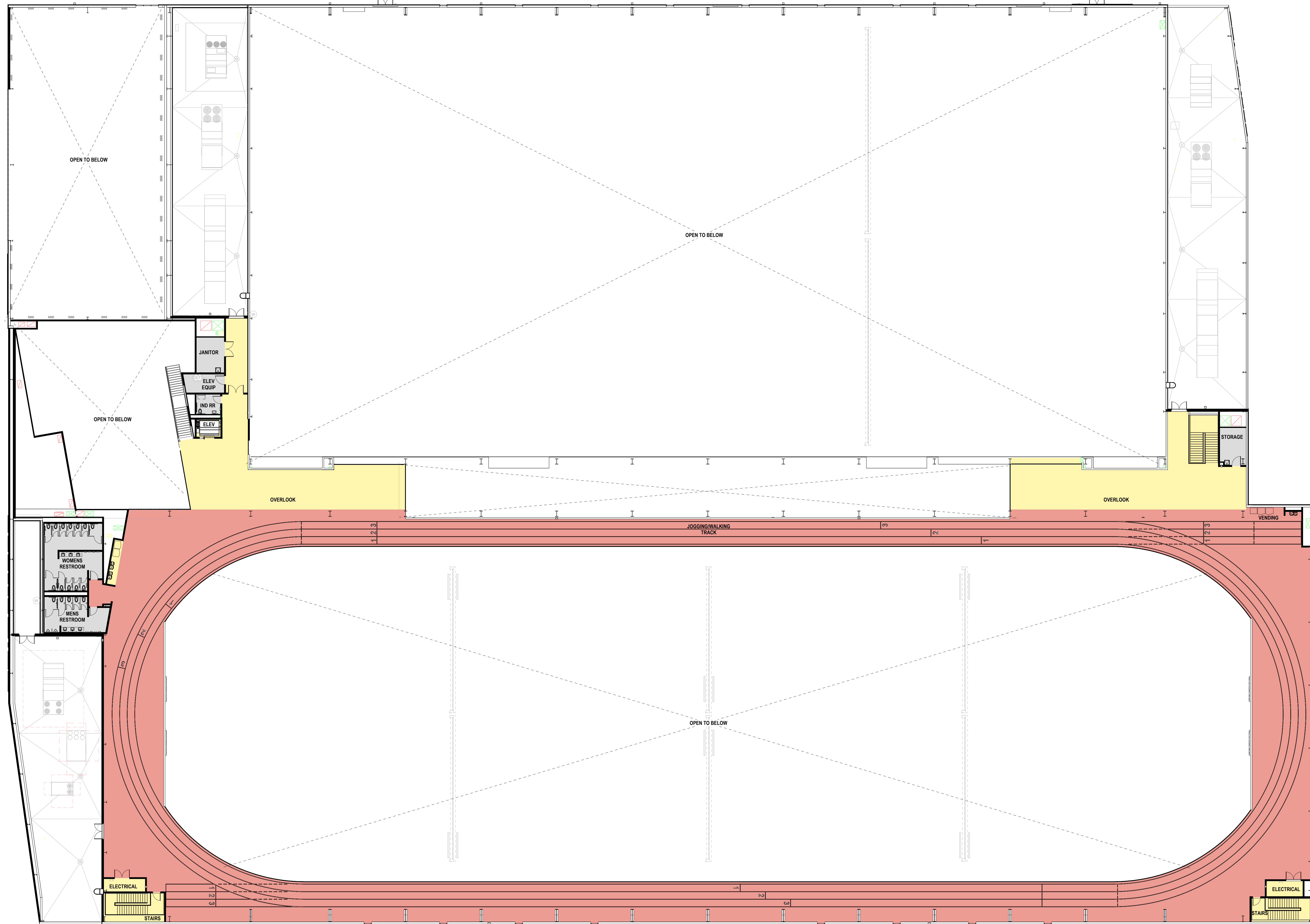
SECOND LEVEL FLOOR PLAN
